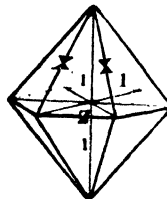
[01 \bar{1} 1]
